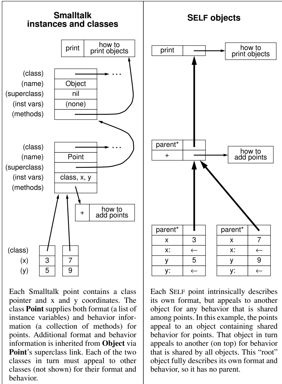
Figure 1. A comparison of Smalltalk instances and classes with SELF objects.
